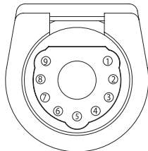
Receptacles seen from mating face
